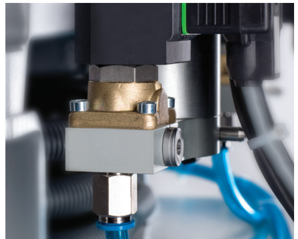
Save time with automatic compressor operation: The newly developed and patented B-DRAIN automatic condensate drain system.
